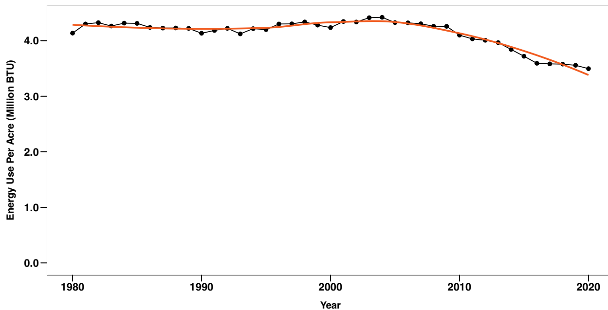
Figure B.17. Energy use (million BTU / acre) for peanuts during 1980-2020
